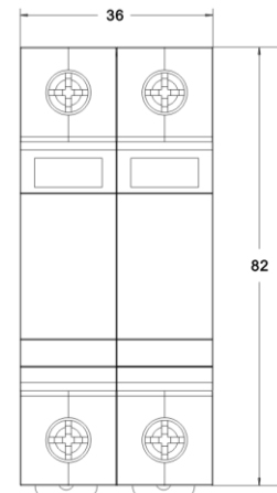
Outline dimension
